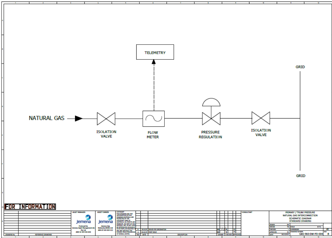
Figure 3: Flow Controlled Interconnection Schematic
