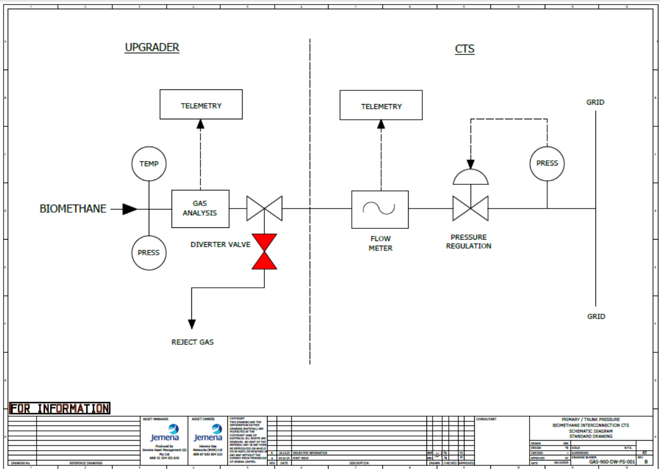
Figure 4: Biomethane Interconnection Schematic
