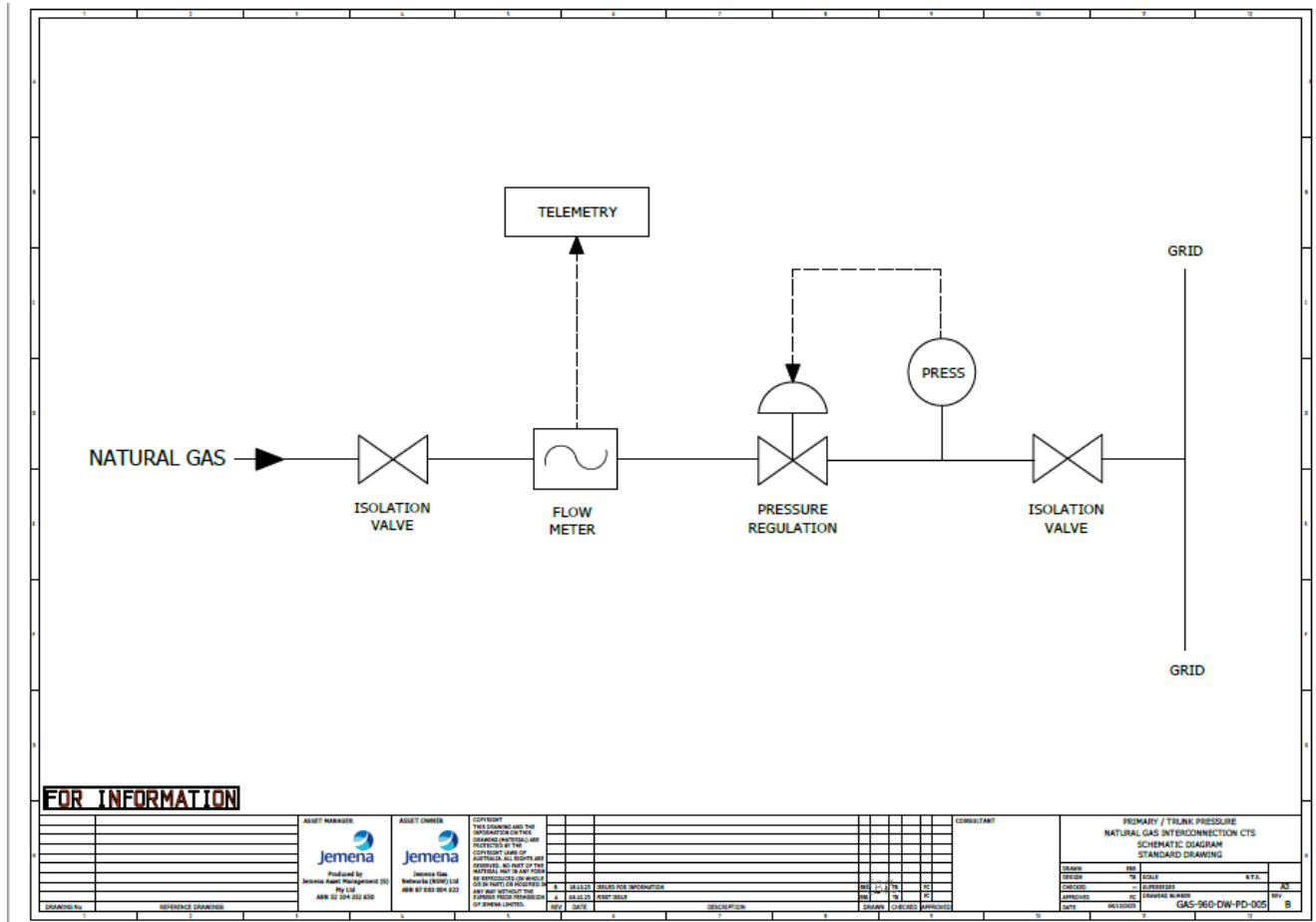
Figure 2: Pressure Controlled Interconnection Schematic
