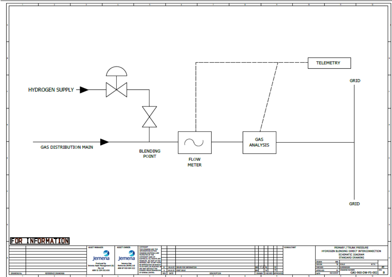
Figure 5: Hydrogen Blending Direct Injection Interconnection Schematic
